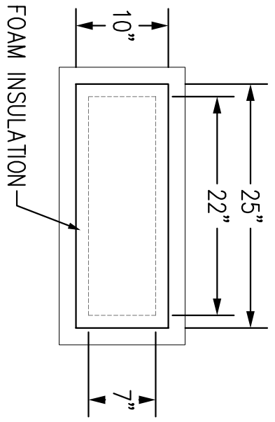
TOP VIEW NOT TO SCALE
